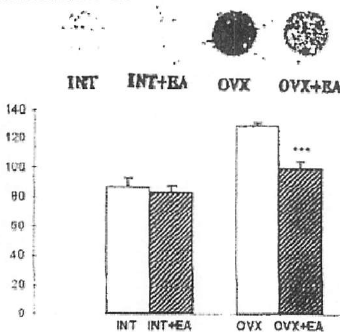
Fig. 5 Effect of EA on expression of ER mRNA in rat brain (dot blot) *** p < 0.01 compared with OVX
